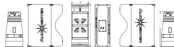
Dimension(WxHxD): 742x302x615mm
