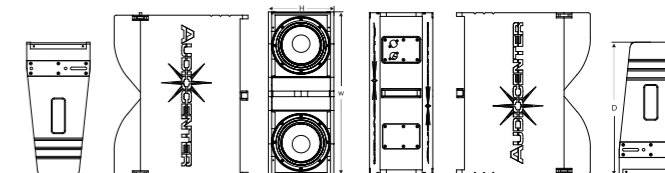
Dimension(WxHxD): 590x236x436mm
