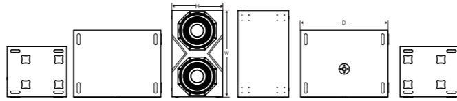
Dimension(WxHxD): 1080x595x760mm
