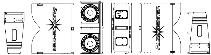
Dimension(WxHxD):590x236x436mm
