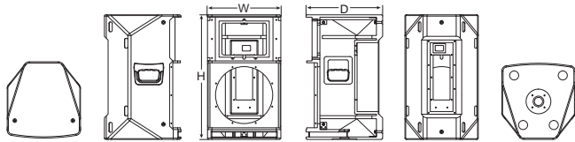
Dimension(WxHxD):356x608x372mm
