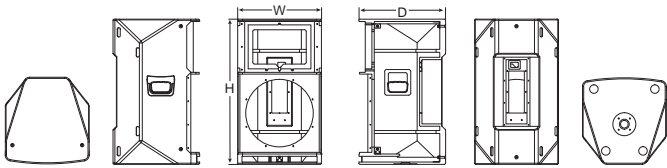
Dimension(WxHxD):439x760x454mm
