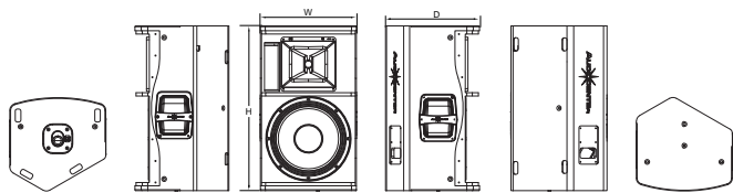
Dimension(WxHxD): 443x726x405mm
