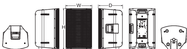
Dimension(W×H×D):381×582×343mm
