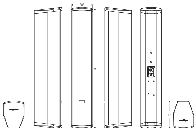
Dimension(W×H×D): 184x1077x255mm
