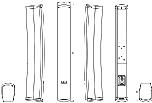
Dimension(W×H×D): 121x918x191mm
