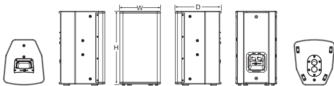
Dimension(WxHxD):245x447x320mm
