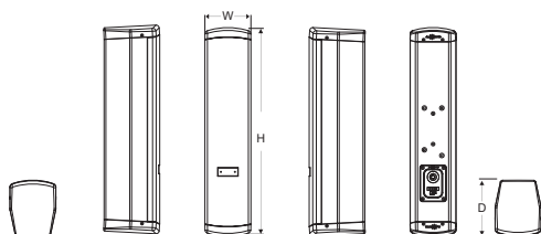
Dimension(W×H×D): 121x549x146mm
