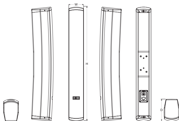
Dimension(W×H×D): 121x918x191mm
